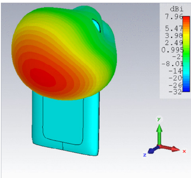
Figure 3: Radiation pattern of the Freevolt antenna inside the CleanSpace tag.
