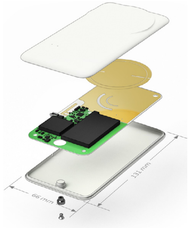
Figure 4: Exploded image of the CleanSpace tag, showing the Freevolt antenna, communication antenna and onboard electronics.
